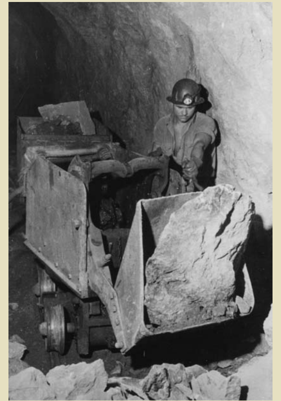
Above: A miner using an air operated Eimco mechanical bogger to clear his drive face after firing a round of explosives underground.
